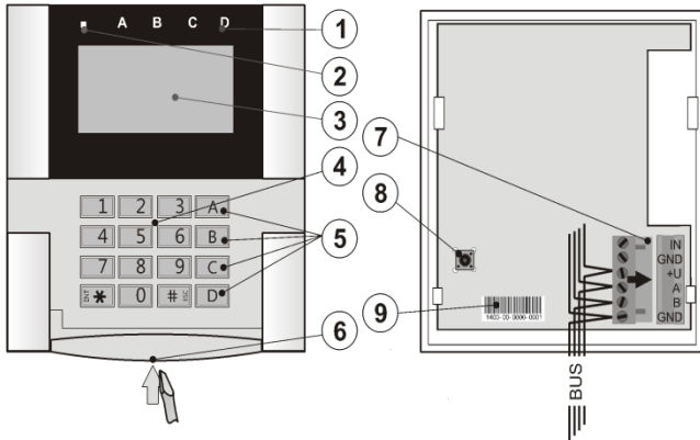
Figure 1: 1 – status indicators; 2 – system indicator; 3 – LCD display; 4 – keypad and the RFID reader; 5 – function buttons A, B, C, D; 6 – keypad opening tab; 7 – detachable BUS terminals; 8 – tamper contact; 9 – production number
