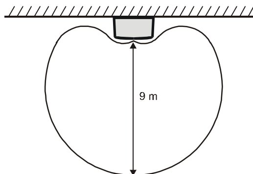
GBS-210 "VIVO" working range diagram
